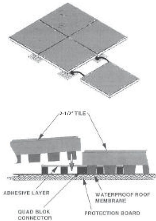
Figure 1. Typical tile field placement
