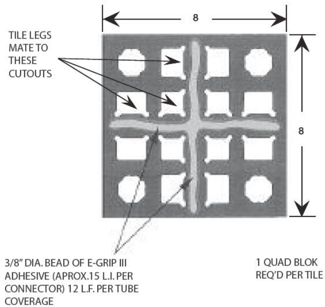
Figure 2. Connector detail
